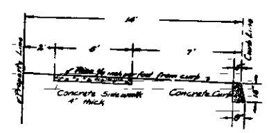
SECTION ON AA Scale 1/2"=1'
