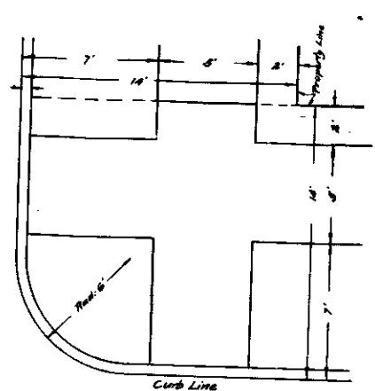
DETAIL AT CORNER Northwest Corner Walnut St. & Mt. Vernon Ave. Scale 1/2"=1'
