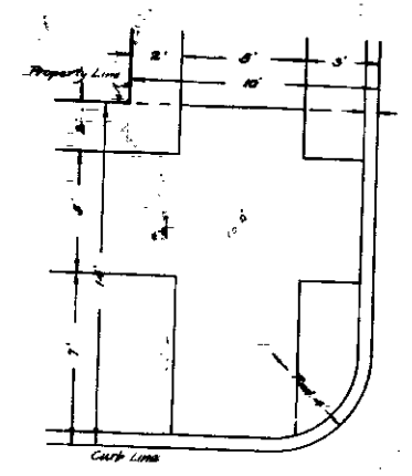
DETAIL AT CORNER Scale 1/2"=1'
